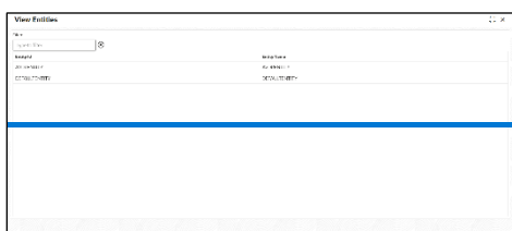
Figure 3: View Entities
